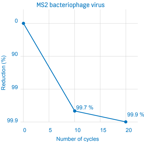
In escalator equipped with KONE Handrail Sanitizer Premium 99.7% of MS2 virus was reduced in 10 cycles and >99.9% in 20 cycles.
