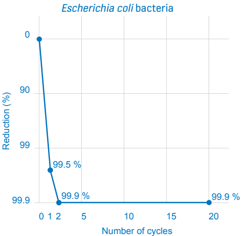
In escalator equipped with KONE Handrail Sanitizer Premium 99.5% of Escherichia coli bacteria was reduced in 1 cycle and >99.9% in 2 cycles.
